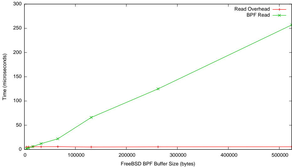
FreeBSD BPF Read Overhead
